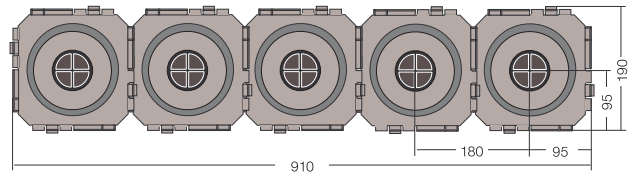
KD 110-2x5-K2/(L)
